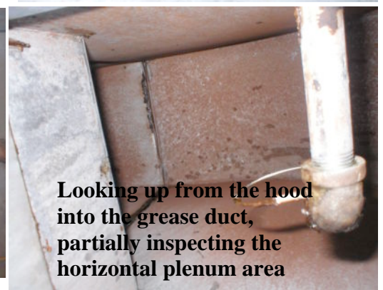
Looking into a horizontal above A hood drop-(notice the additional ductwork beyond the curve).
